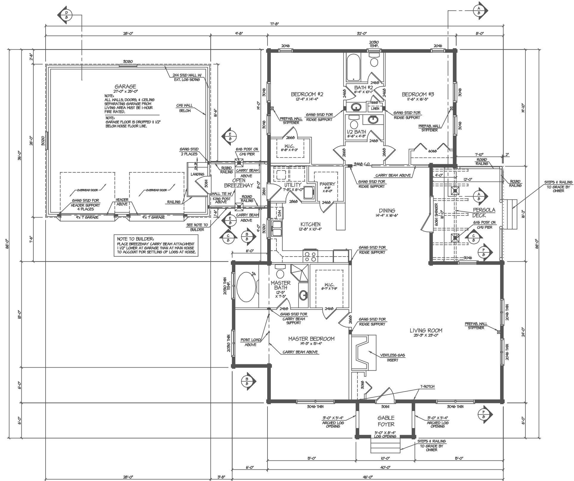
1st FLOOR PLAN 3/32" = 1'-0"
