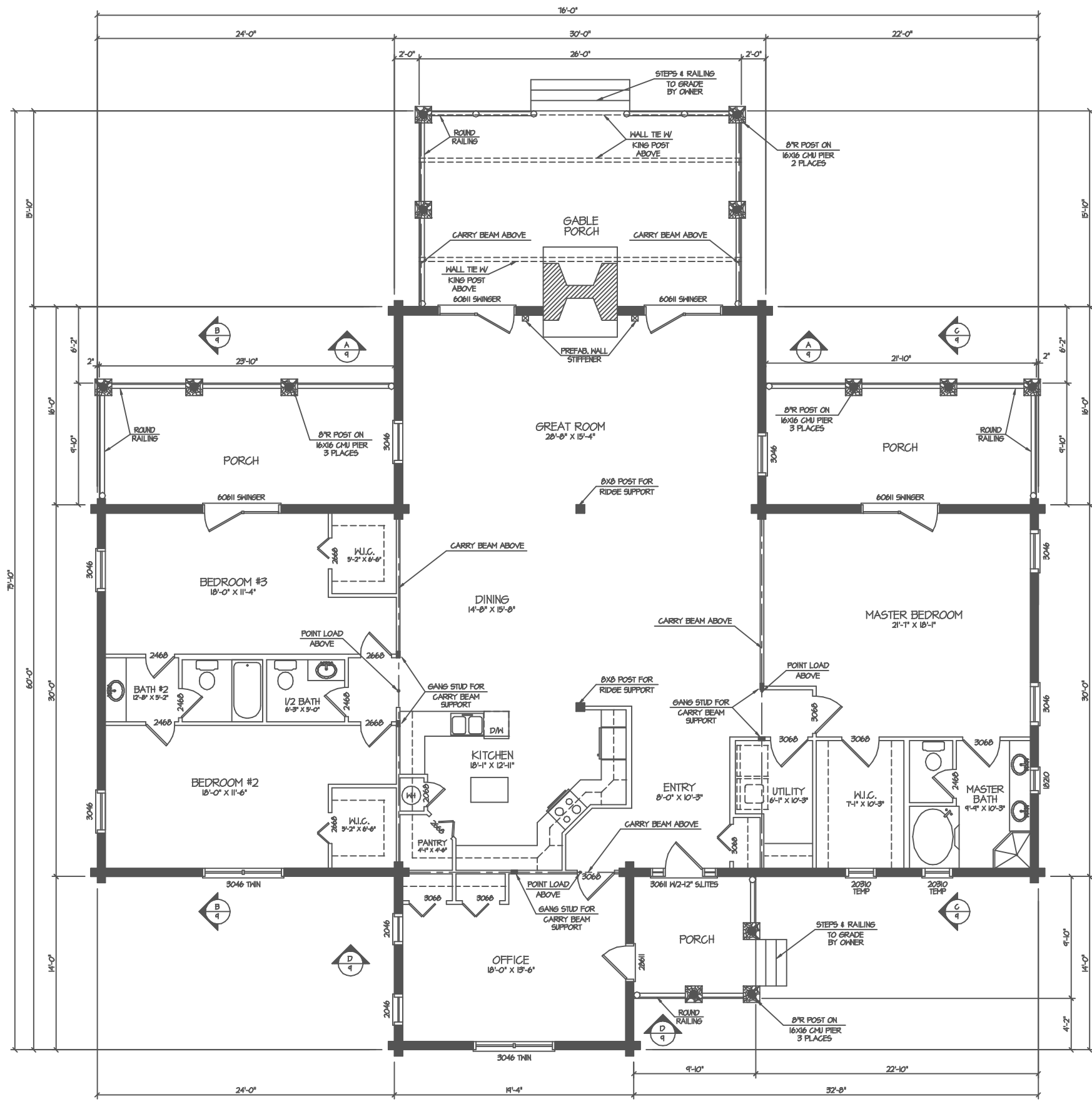
1st FLOOR PLAN 3/32" = 1'-0"
