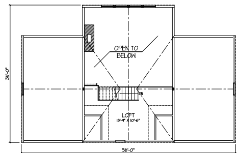
2nd Floor Plan (266 S.F.)
