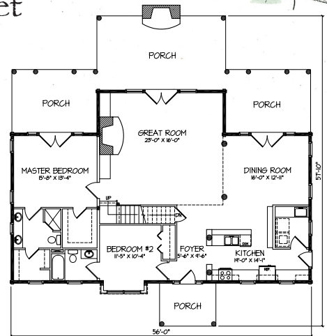
1st Floor Plan (1,775 S.F.)
