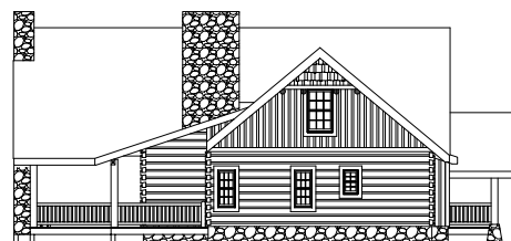
Left Elevation
