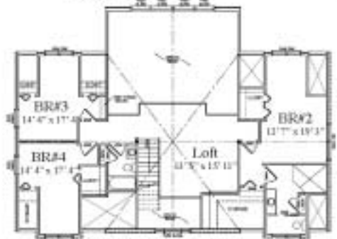
2nd FLOOR PLAN (1,166 S.F.)
