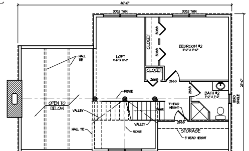
2nd Floor Plan (532 S.F.)
