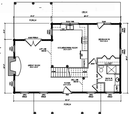
1st Floor Plan (956 S.F.)
