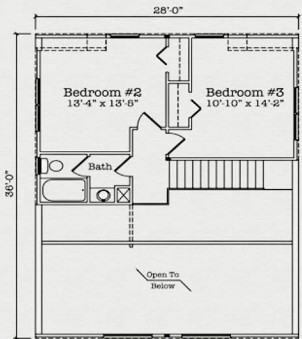
Floor Plan "A"
