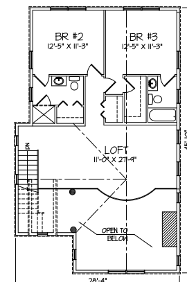
2nd Floor Plan (867 S.F.)
