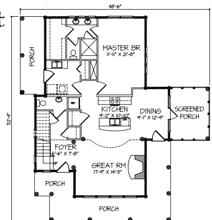
1st Floor Plan (1,290 S.F.)
