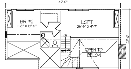
2nd Floor Plan (463 S.F.)
