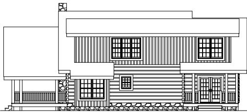
Rear Elevation
